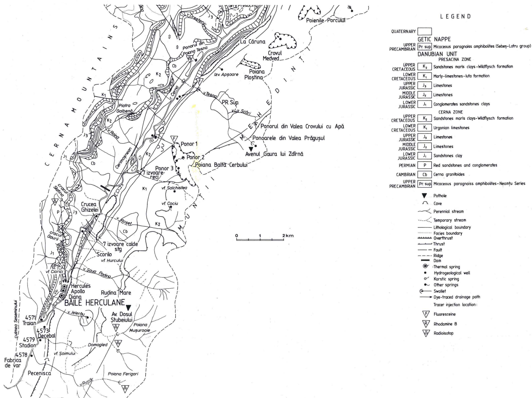
Figure 1. - Central part of a hydrogeological map of the Cerna valley (geology after S. Năstăseanu and I. Bercia).
